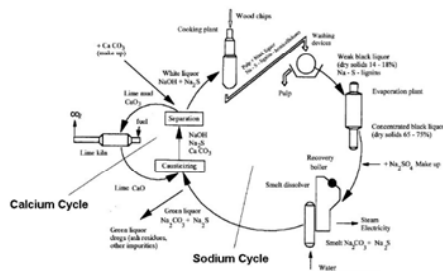
Pic3- Ca and Sodium Cycle in Recovery plant Adapted from European Commission IPPC 2001
